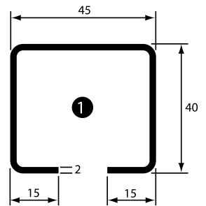
Top Track
